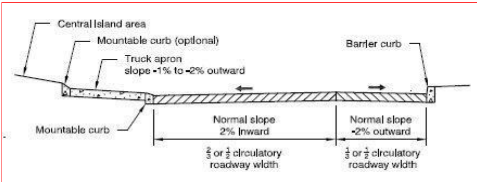
c/s of road in built-up area
