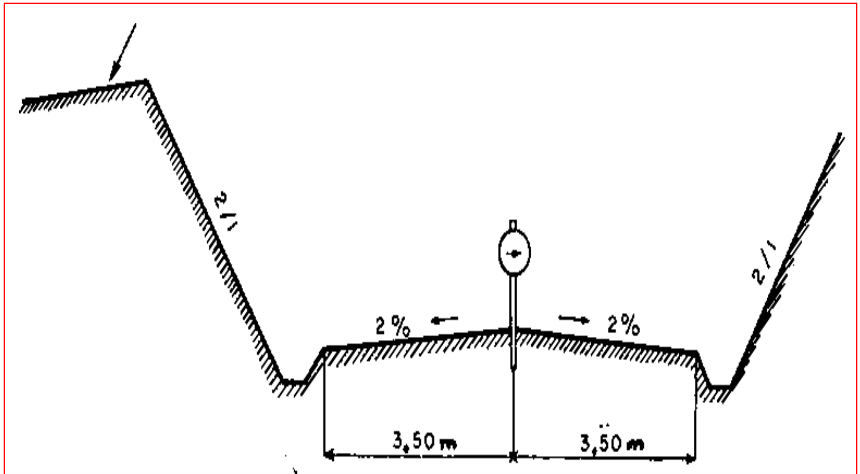
c/s of road in cutting
