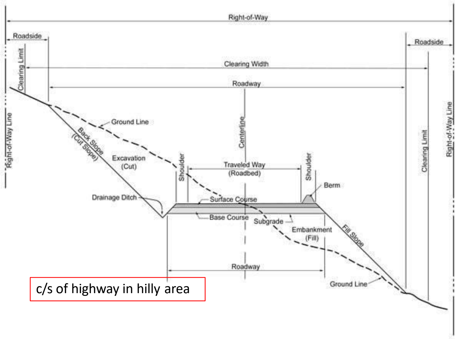
Typical Road Section
