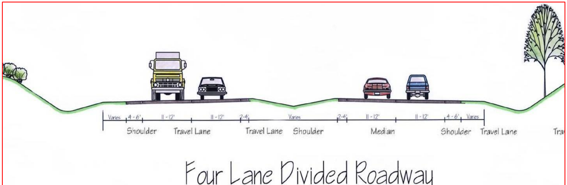
c/s of road in built-up area
