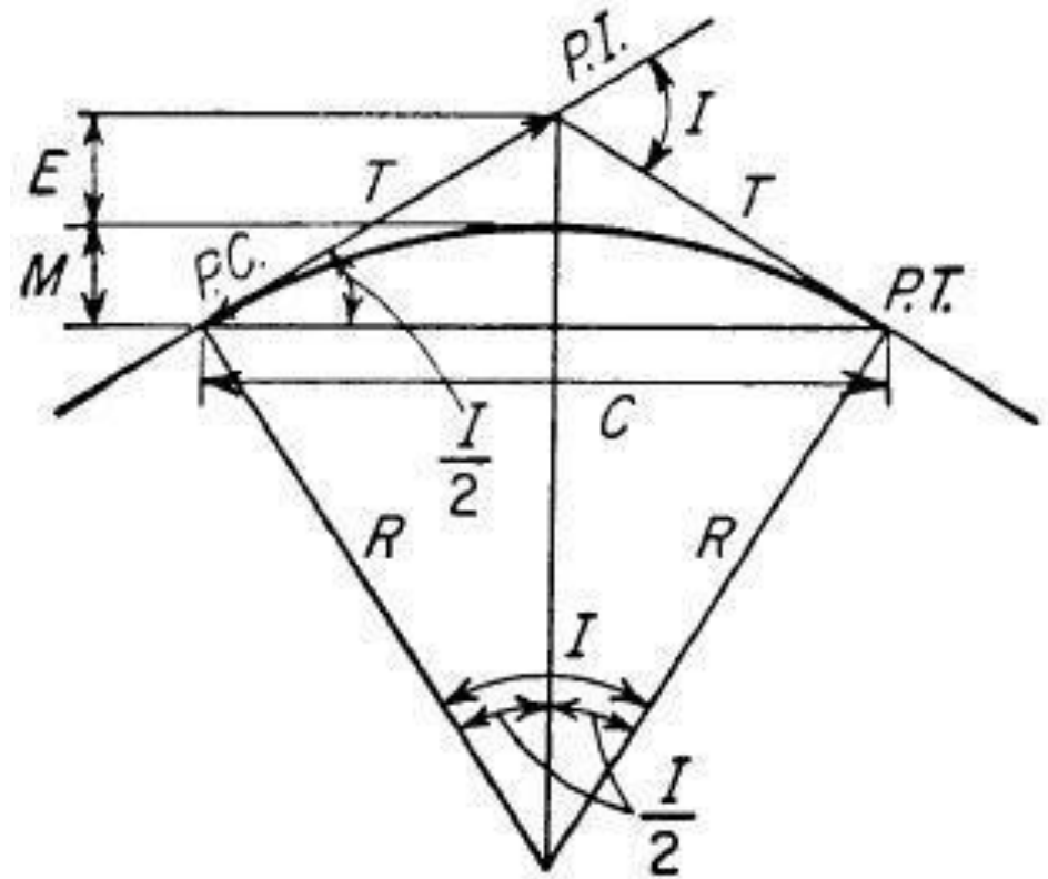
Circular curve.
